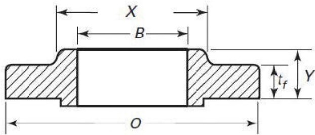
Slip-On Welding
